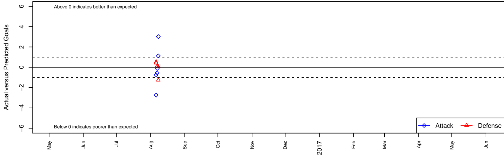
San Jose Earthquakes PDA B03 Dots are actual minus expected GF (blue circles) and GA (red triangles). Blue line is smoothed change in attack strength. Red is smoothed change in defense strength.
